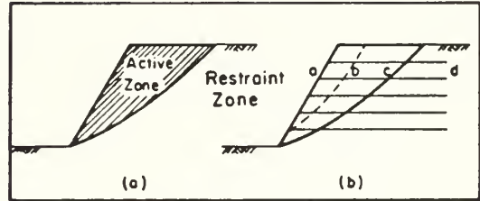
Fig. 7 Modes of Failure
